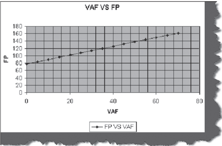
FIGURE 158 FP versus VAF
